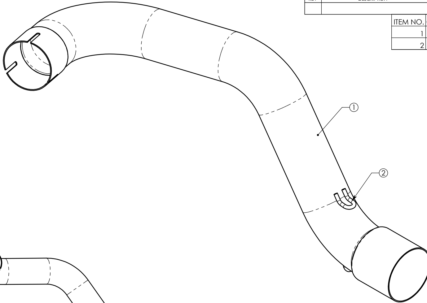
FRONT VIEW 1:4
